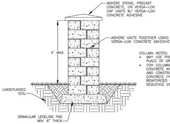
20" STANDARD COLUMN SECTION STANDARD-UNREINFORCED COLUMN (4' TALL MAX.) SCALE: NONE
