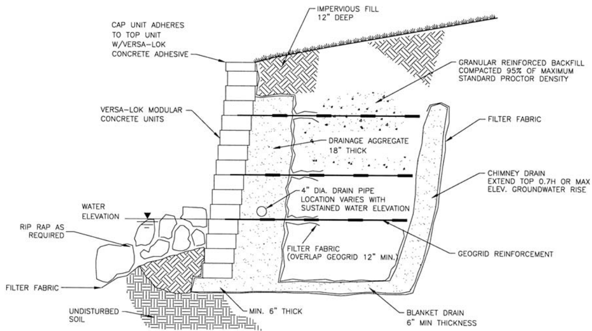
TYPICAL SECTION—REINFORCED SHORELINE WALL
