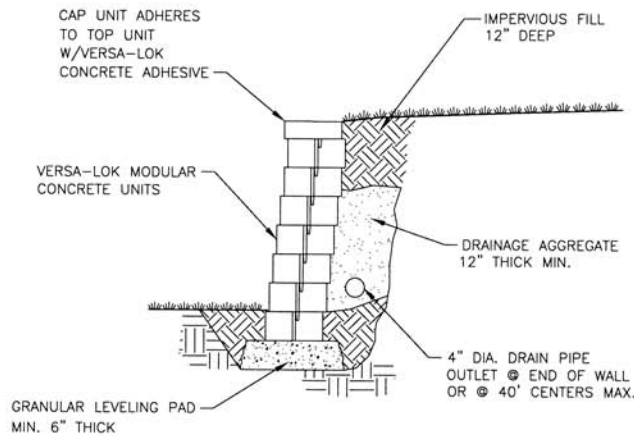
TYPICAL SECTION—UNREINFORCED RETAINING WALL
