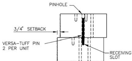
Pinning Detail
