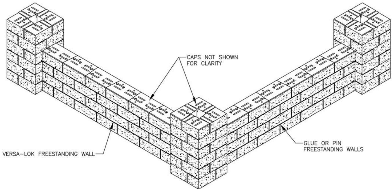
COLUMNS WITH FREESTANDING WALLS COLUMNS SCALE: NONE
