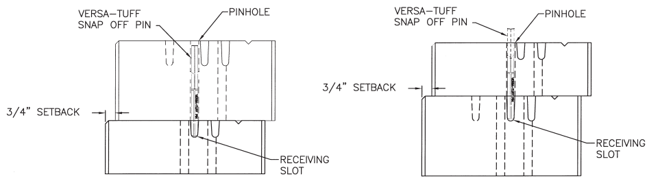
PINNING DETAIL
