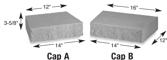
Matching cap units attractively finish VERSA-LOK walls.
